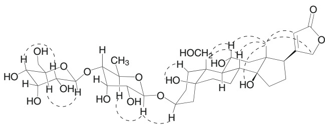
Figure 2. Key ROESY correlations of 1 .
